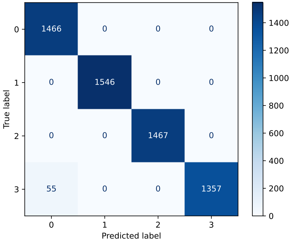
Fold 4 - Confusion Matrix
